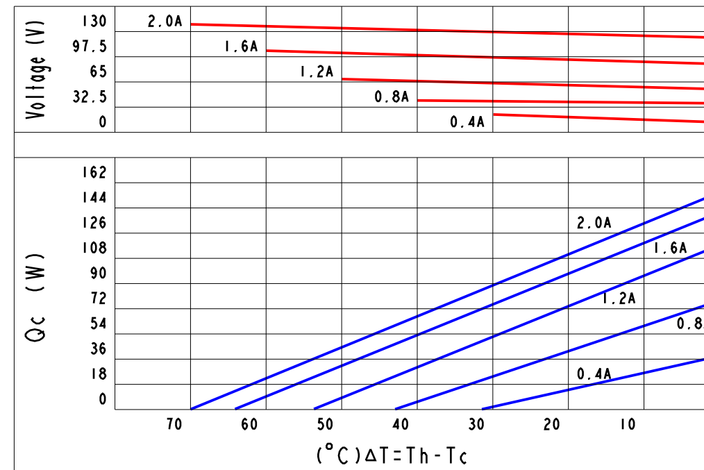
Curve Chart(Be Confined To TEC1-1041028484):
