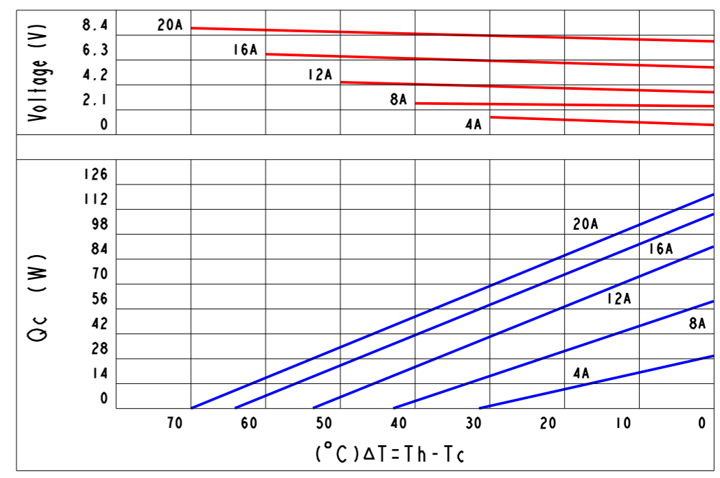
Curve Chart(Be Confined To TEC1-071204447):
