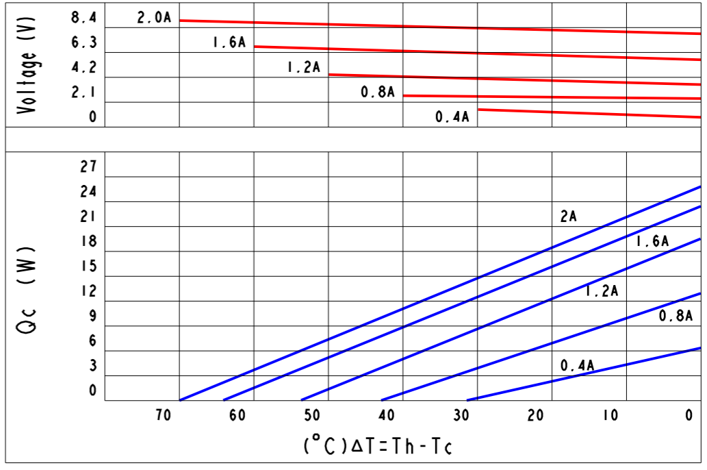
Curve Chart(Be Confined To TEC1-071021818):
